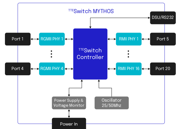
Block diagram of components in TTESwitch Mythos
